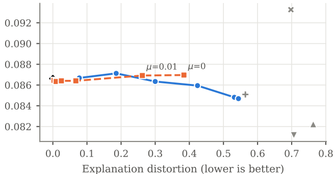
Credit Card Fraud (DNN + LIME)
