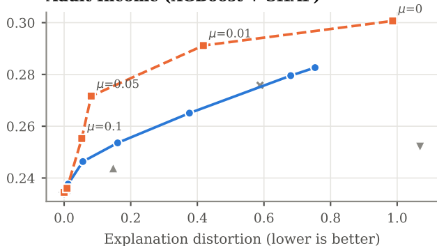
Adult Income (XGBoost + SHAP)
